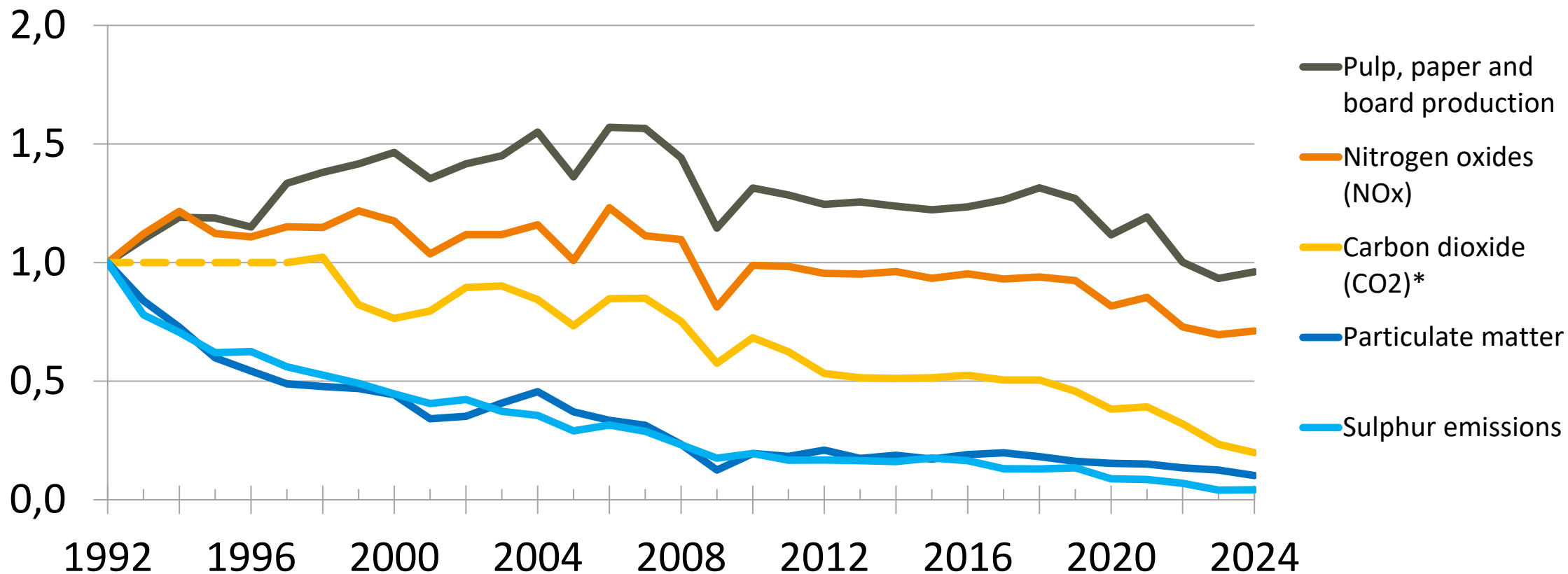
Emissions from the pulp and paper industry indexed to air
